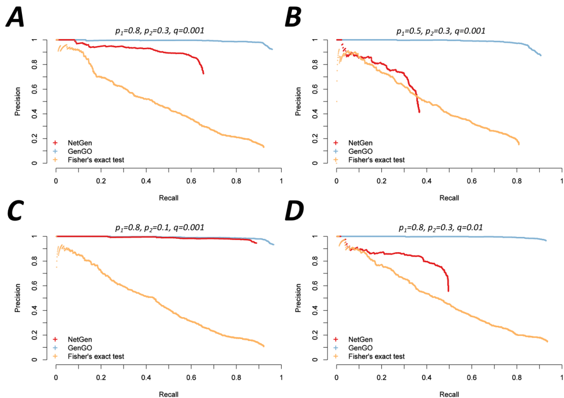
Figure S5. The performance of NetGen and alternative methods on biological process (BP) domain. Each panel stands for a setting of generating parameters. The performance of NetGen, GenGO and Fisher's exact test are shown in red, blue and orange respectively. The active gene lists were simulated under the assumption of GenGO.
