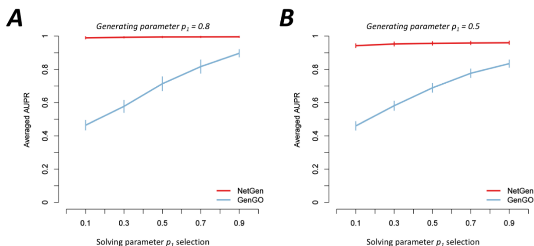
Figure S1: Sensitivity analyses results of p_1 . (A) p_1 = 0.8 and (B) p_1 = 0.5 were selected for generating simulated samples. The performances of NetGen and GenGO were compared using the averaged AUPR plus/minus one-fold standard deviation at different values of solving parameter p_1 . The results of NetGen and GenGO were shown in red and blue curve, respectively.
